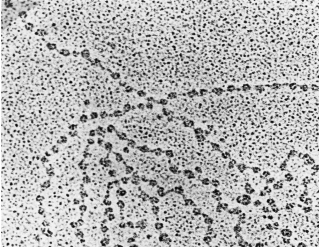
Electron micrograph of chromatin showing nucleosomes
