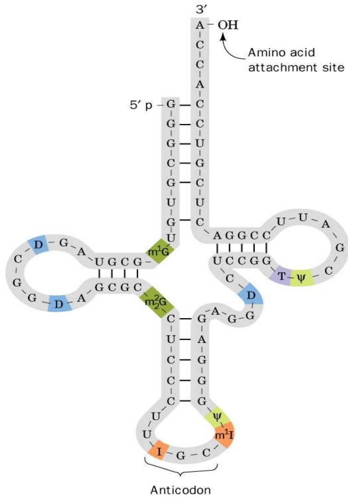
Structure of a tRNA
