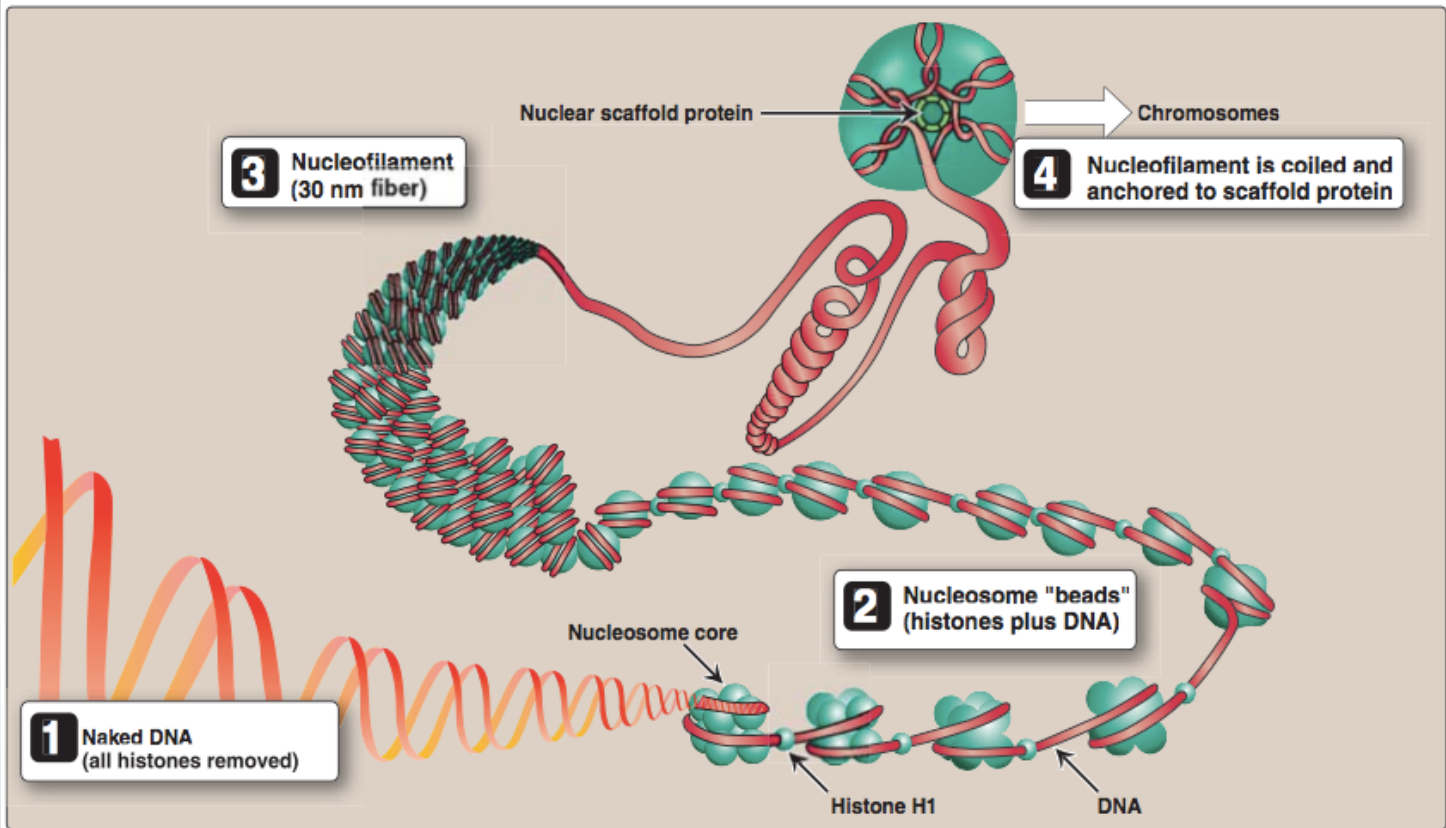
Chromatin filament with nucleosomes and naked DNA
