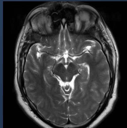
MRI T2WI
