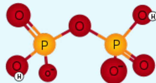
Pyrophosphate
