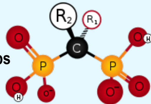
Bisphosphonate
