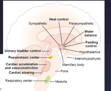
Figure 60-5 Autonomic control areas in the brain stem and hypothalamus.
