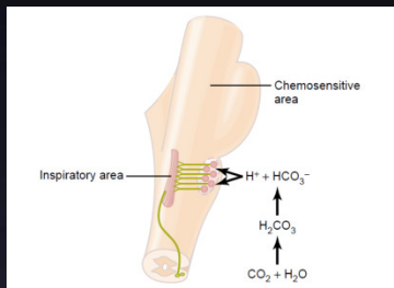
Figure 41-2 Stimulation of the brain stem inspiratory area by signals from the chemosensitive area located bilaterally in the medulla, lying only a fraction of a millimeter beneath the ventral medullary surface. Note also that hydrogen ions stimulate the chemosensitive area, but carbon dioxide in the fluid gives rise to most of the hydrogen ions.
