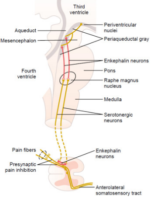
Figure 48-4 Analgesia system of the brain and spinal cord, showing (1) inhibition of incoming pain signals at the cord level and (2) presence of enkephalin-secreting neurons that suppress pain signals in both the cord and the brain stem.
