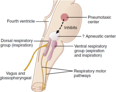
Figure 42-1. Organization of the respiratory center.
