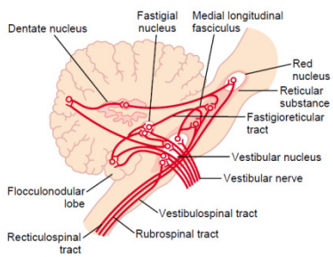
Figure 55-13 Connections of vestibular nerves through the vestibular nuclei (the large oval white area) with other areas of the central nervous system.
