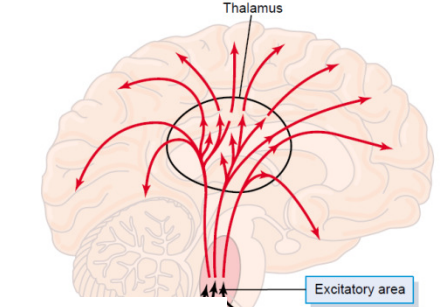
Excitatory area 5th Cranial nerve Inhibitory area
