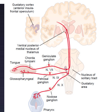
Figure 53-2 Transmission of taste signals into the central nervous system.
