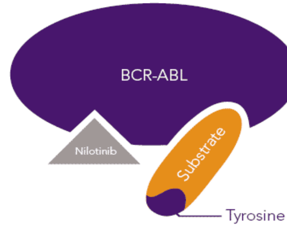
Inactivated BCR-ABL
