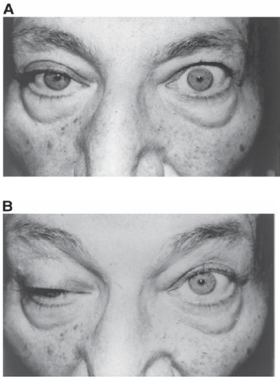
Fig. 1. (A) The patient is attempting to look up, evidenced by the contraction of the frontalis muscle. Note the slight right ptosis and left lid retraction. (B) Lid fatigue that developed during the sustained upward gaze, manifested by marked ptosis on the right, and lessening of the lid retraction on the left. (Photos courtesy of Dr. J. Lawton Smith.)
