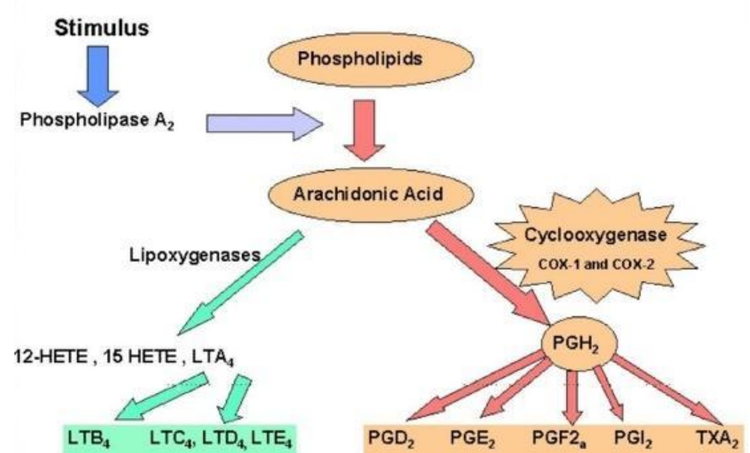
Figure 2 : Biosynthesis of eicosanoids
